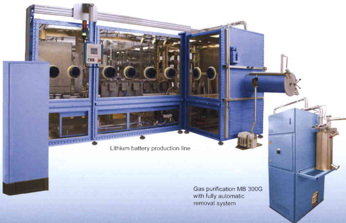
PLC controlled gas purification system
